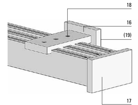
Wall bracket with end cap
