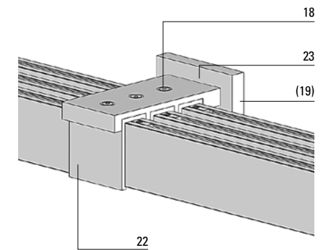
Rail connector
